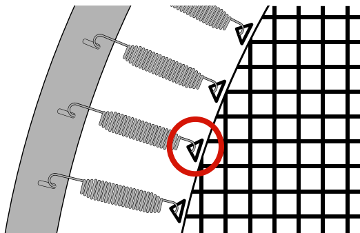
Spring attachments on a polymesh trampoline bed
